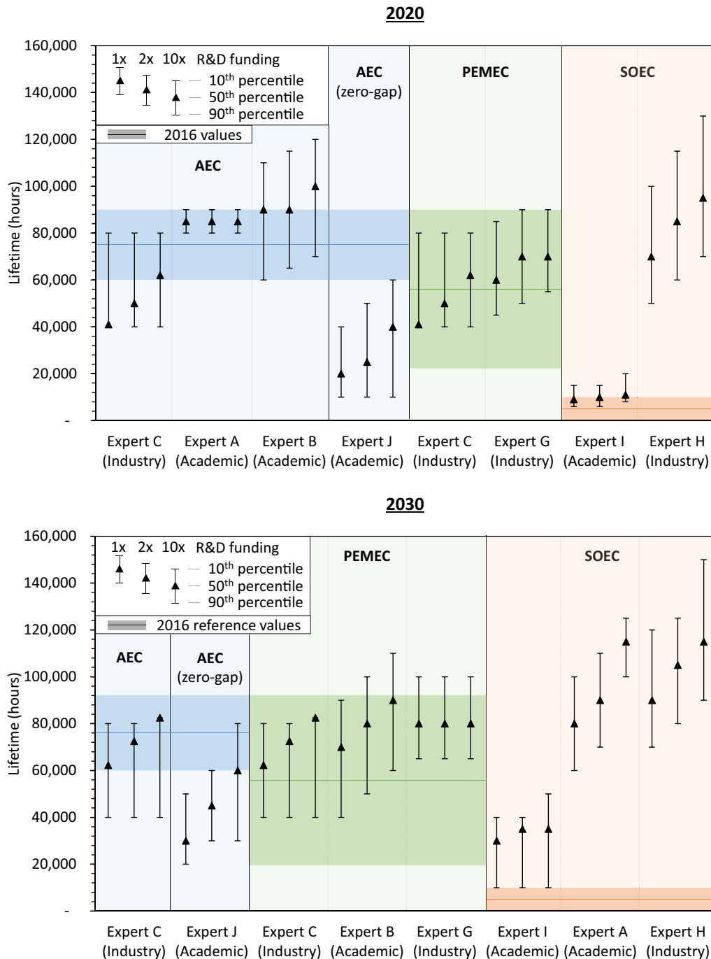
Fig. 5 – Elicited expert estimates for 2020 and 2030 lifetime (in hours) as a function of R&D funding (1x, 2x, 10x). Data points indicate 50th, uncertainty bars 90th and 10th percentile estimates. Expert C made estimates for AEC and PEMEC. Expert J made estimates for AEC zero gap configurations. Results are sorted by technology and in ascending order for 50th percentile estimates. 2016 reference values based on Table 1.
