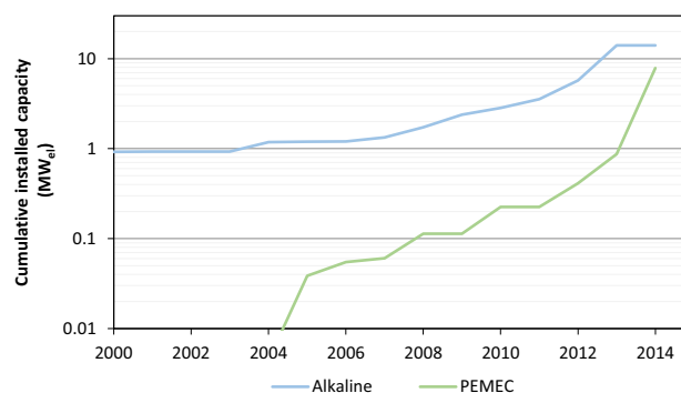
Fig. C.1 – Cumulative installed capacities of AEC and PEMEC systems in Power-to-gas applications (data taken from Ref. [50]).
