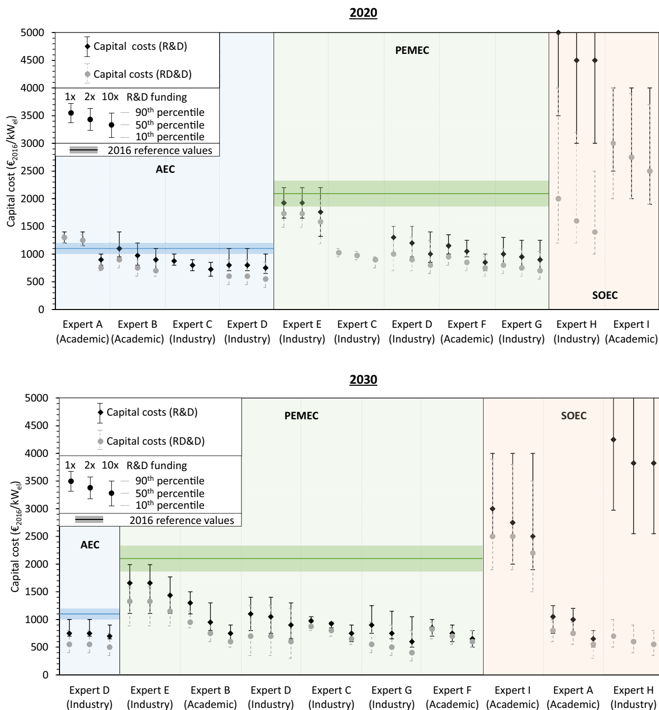
Fig. 3 – Elicited expert estimates for 2020 and 2030 capital costs without (◆ R&D) and with production scale-up (● RD&D) as a function of R&D funding (1x, 2x, 10x). Data points indicate 50th, uncertainty bars 90th and 10th percentile estimates. Expert C made 2020 estimates for AEC (R&D) or PEMEC (RD&D). Expert D made all estimates for AEC and PEMEC. Results are sorted by technology and in descending order for 50th percentiles without production scale-up (◆ R&D). 2016 reference values based on Table 1. No 2016 reference values for SOEC as this technology is not yet widely commercialised.
