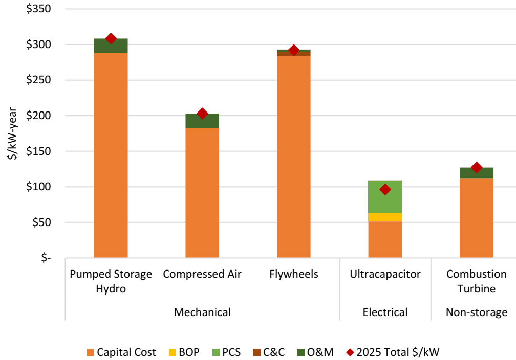
Figure 5.4. Annualized $/kW cost of non-battery technologies.
